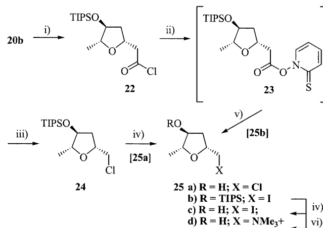
Scheme 3. i) (COCl) 2 , DMF (cat.), pyridine, C 6 H 6 , 0^\circ\text{C} , 3 h; ii) 2-mercaptopyridine N -oxide sodium salt, DMAP (cat.), CCl 4 ; iii) 65^\circ\text{C} , 1.5 h, 73% from 20b ; iv) TBAF, THF, 20^\circ\text{C} , 40 h, 60%; v) as ii) but CHI 3 in place of CCl 4 and reflux in cyclohexene for 15 h, 60% from 20b ; vi) Me 3 N, EtOH, 70^\circ\text{C} , 4 h (sealed tube), 75%
