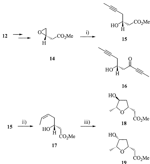
Scheme 1. i) Lithiopropyne, \text{BF}_3 \cdot \text{OEt}_2 , THF, -78^\circ\text{C} , 4 h, 80% 15 + 5–10% 16 ; ii) \text{H}_2 (1 atm.), 5% Pd-BaSO 4 , quinoline, EtOAc, 0.75 h, 87%; iii) \text{I}_2 , NaHCO 3 , MeCN, 0-5^\circ\text{C} , 72 h, 63% 18 + ca. 11% 19
