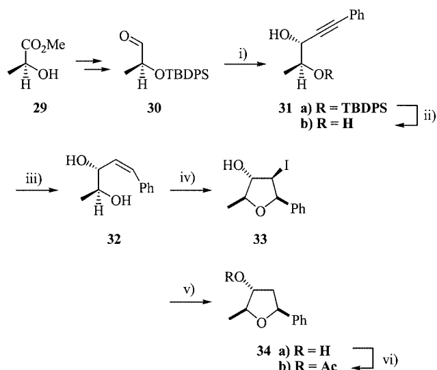
Scheme 4. i) Lithiophenylacetylene, 12-crown-4, THF, -78^{\circ}\text{C} to 0^{\circ}\text{C} , 4 h, 76% (+ 11% of the syn -isomer); ii) TBAF, THF, 20^{\circ}\text{C} , 2 h, 93%; iii) H 2 (1 atm.), 5% Pd-CaCO 3 , quinoline, hexane/2% MeOH, 20^{\circ}\text{C} , 2 h; iv) I 2 , NaHCO 3 , MeCN, 0^{\circ}\text{C} , 4 h, 51% from 31b ; v) H 2 (1 atm.), 10% Pd-C, Et 3 N, EtOAc, 20^{\circ}\text{C} , 16 h, 98%; vi) Ac 2 O, pyridine, 20^{\circ}\text{C} , 16 h, 97%
