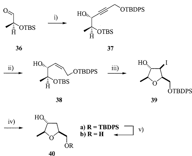
Scheme 6. i) \text{LiC}\equiv\text{CCH}_2\text{OTBDPS} , 12-crown-4, THF, -78^\circ\text{C} to 0^\circ\text{C} , 4 h, 65% (+ 9% of the syn isomer); ii) \text{H}_2 (1 atm.), 5% Pd- \text{CaCO}_3 , quinoline, MeOH, 20^\circ\text{C} , 0.25 h, 90%; iii) \text{IBr} , \text{NaHCO}_3 , MeCN, -10^\circ\text{C} , 3.5 h, 68%; iv) \text{H}_2 (1 atm.), 10% Pd-C, \text{Et}_3\text{N} , EtOAc, 20^\circ\text{C} , 16 h, 91%; v) \text{NH}_4\text{F} , MeOH, 20^\circ\text{C} , 16 h, 56%
